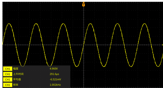
Figure 22 Oscilloscope Acquisition AO Signal
