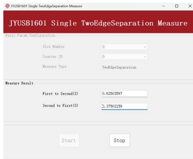
Figure 35 Two-EdgeSeparation Measure for Single Mode
