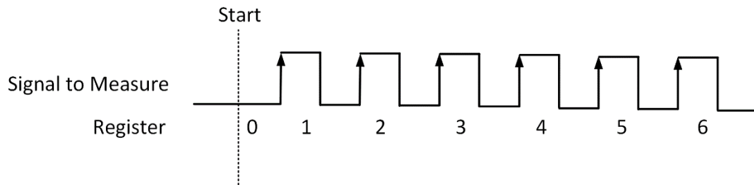
Figure 25 Simple Edge Counting in Single Mode
