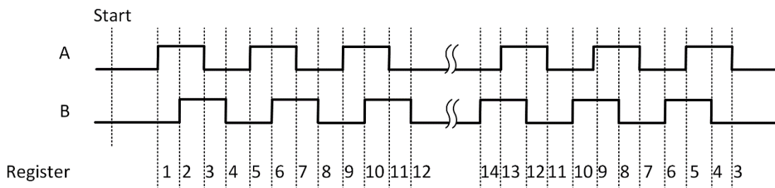
Figure 37 Quadrature Encoder x4 modeTake Encoding x2 mode as an example.
