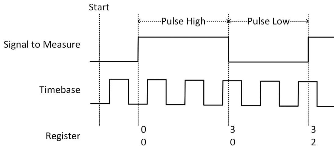
Figure 28 Pulse Measurement in Single Mode
