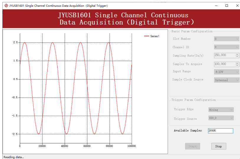
Figure 9 Digital Trigger Acquisition
