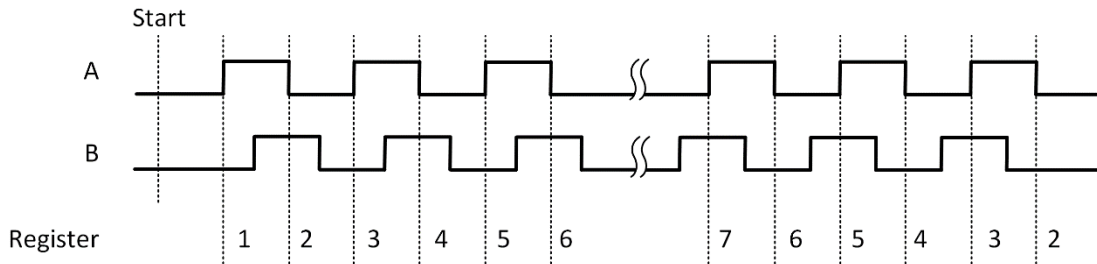
Figure 36 Quadrature Encoder x2 Mode
