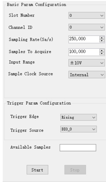
Figure 8 Digital Trigger Parameters
