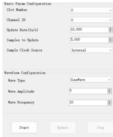
Figure 15 AO Continuous NoWrapping Output Parameters
