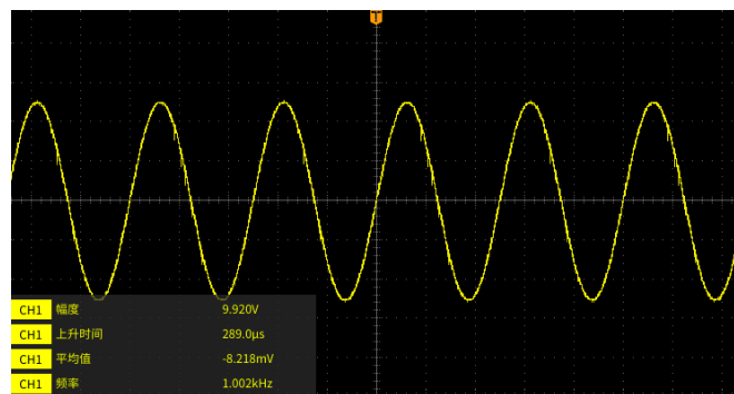
Figure 14 Oscilloscope Acquisition Signal
